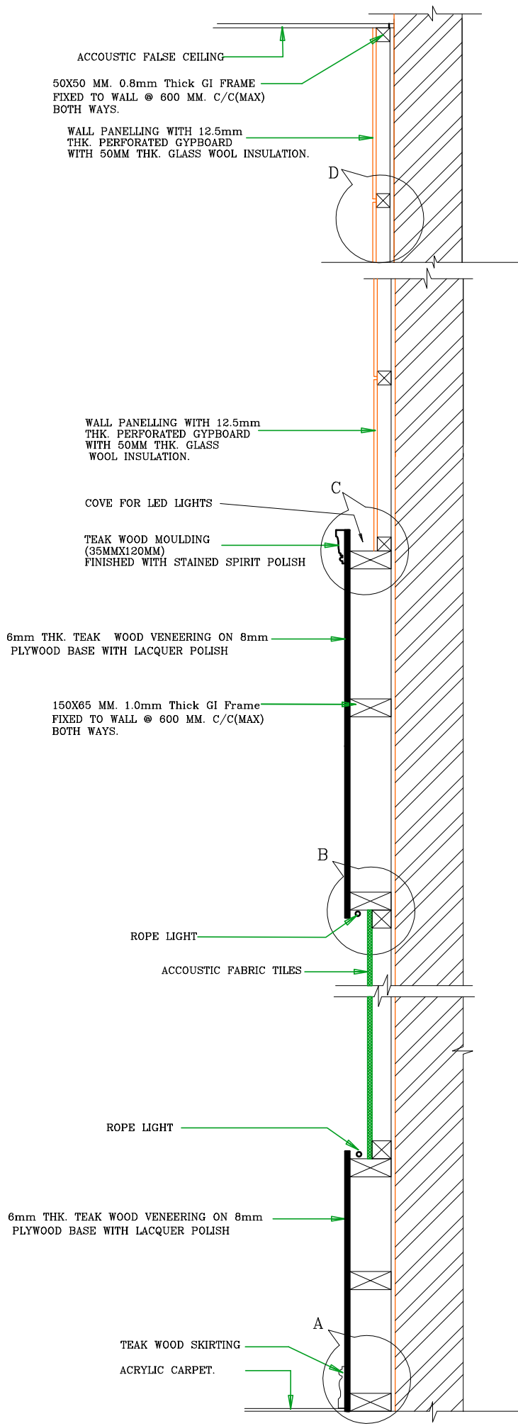
SECTION AT Y-Y. SCALE-1:10
