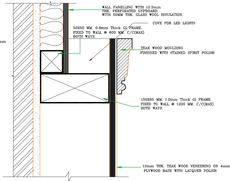
DETAIL AT C SCALE-1:2
