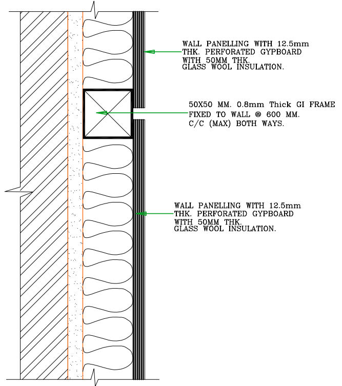
DETAIL AT D SCALE-1:2
