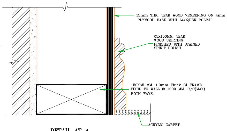
DETAIL AT A SCALE-1:2
