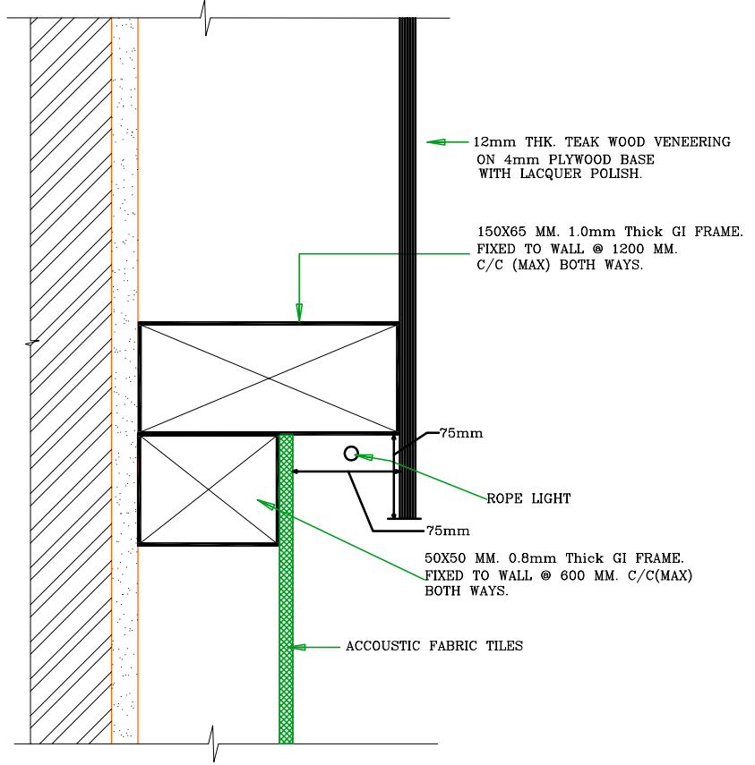
DETAIL AT B SCALE-1:2
